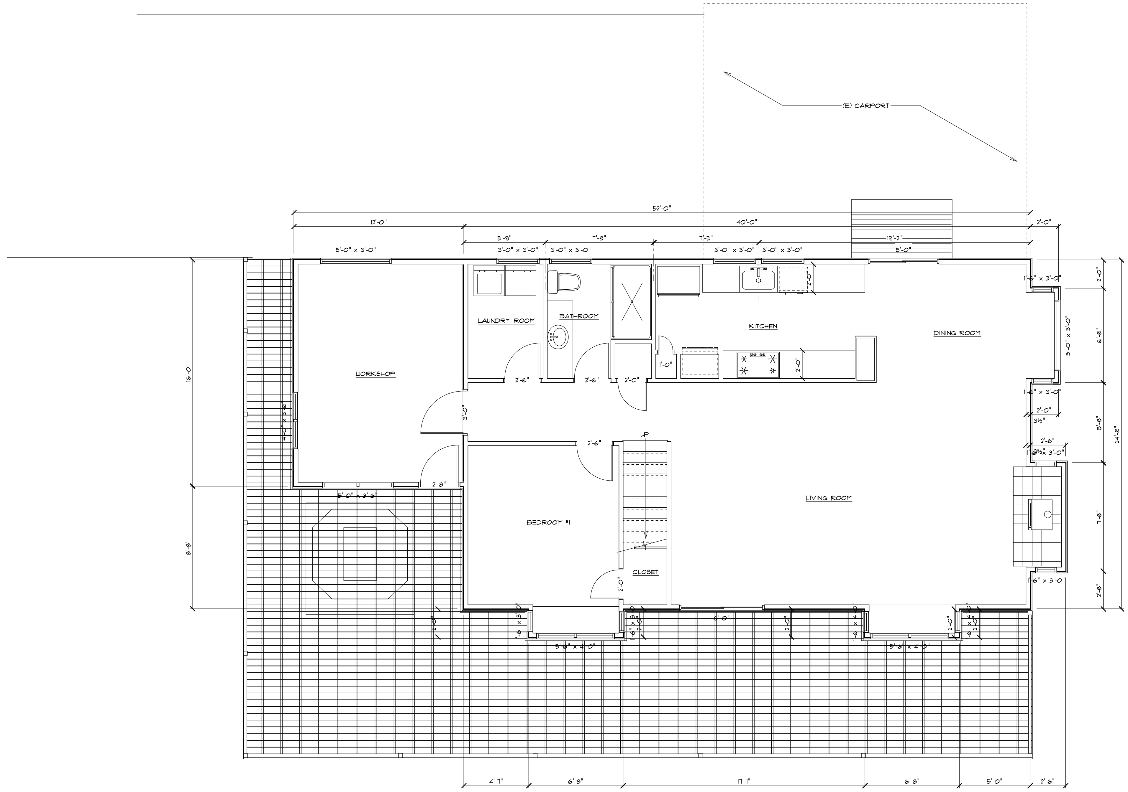
LOW FLOORPLAN @ 1/4" = 1'-0"
