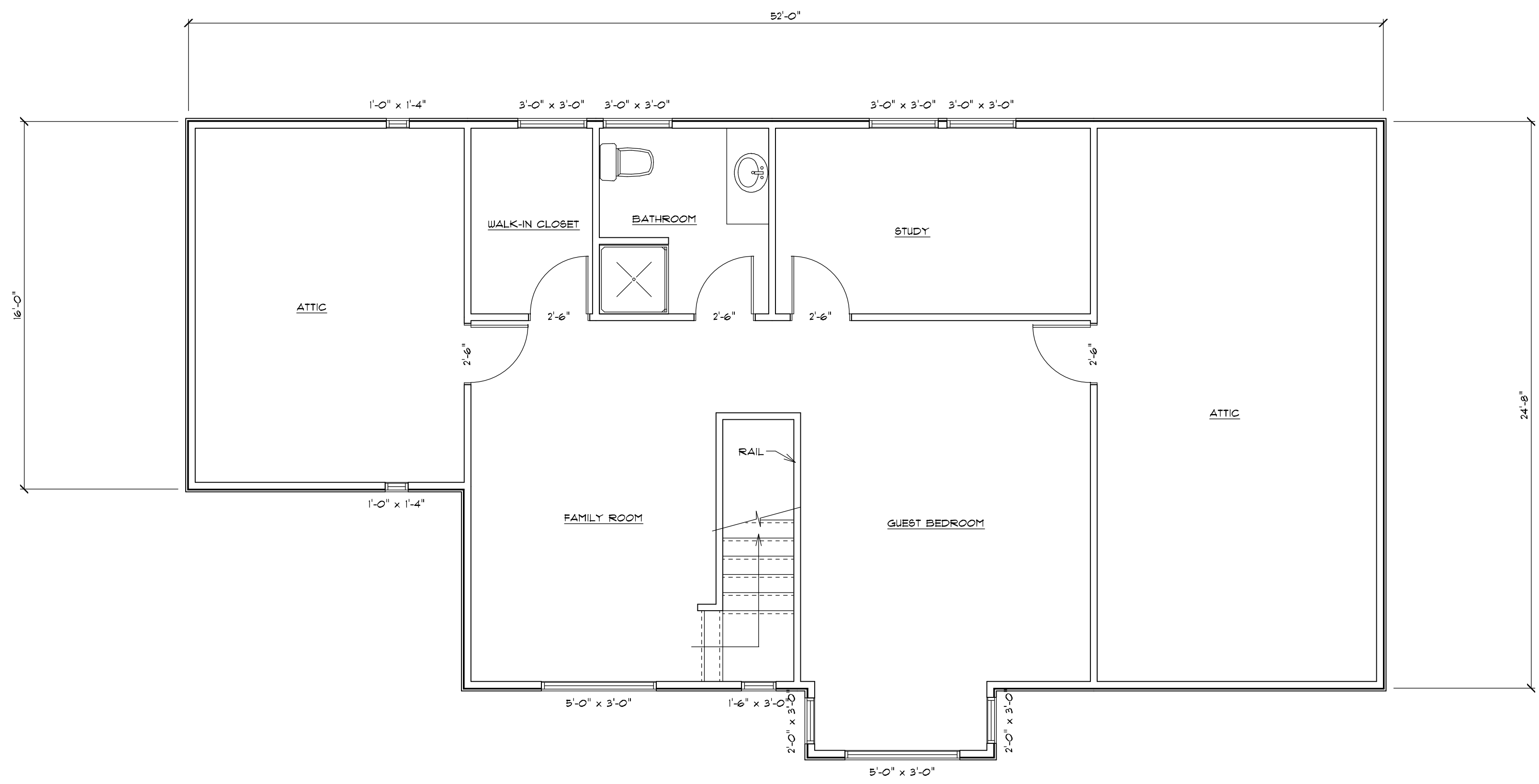
UPPER FLOOR PLAN @ 1/4" = 1'-0"
